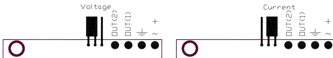
Figure 4. The upper part of the eSense PCB seen from the back with the jumper in voltage (default) or current position.
