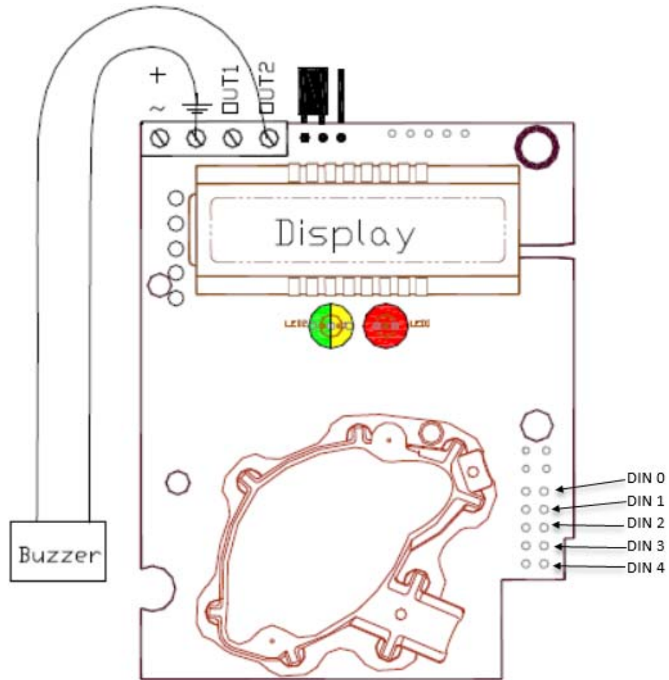
Figure 3. The eSense PCB
