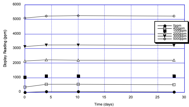
Fig. 6-1 - Durability of FG-010 against H 2 S
