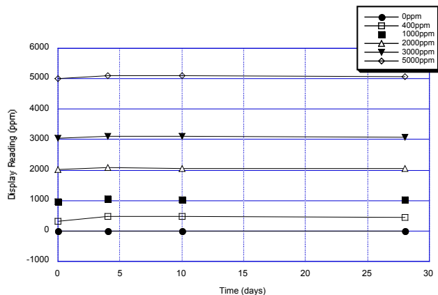
Fig. 6-2 - Durability of FG-010 against SO 2
