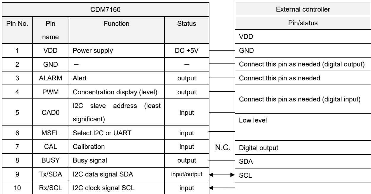
Operation sequence from the viewpoint of the External Controller (master) Connection
