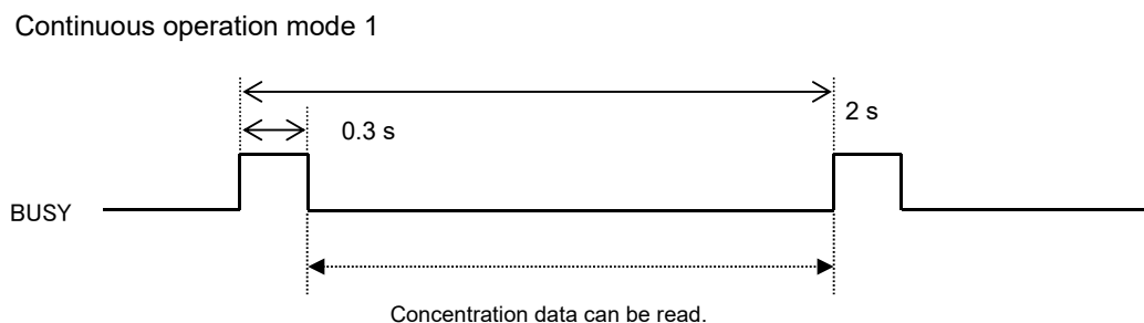
Figure 3 - Continuous Operation Mode
