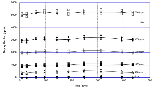
Fig. 5 - Long term stability of FG-010
