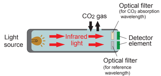
Fig. 2 - Basic structure of FG-010 optics
