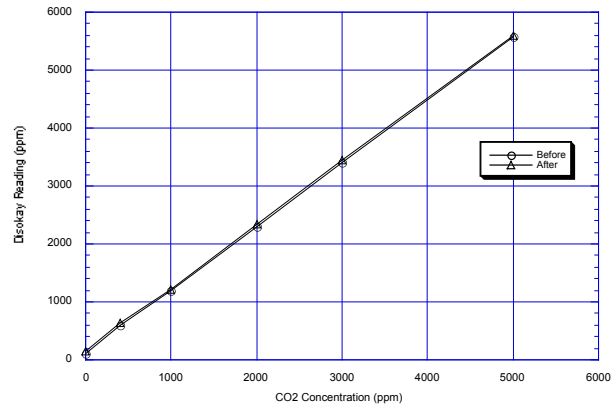
Fig. 7 - Durability of FG-010 against dust
