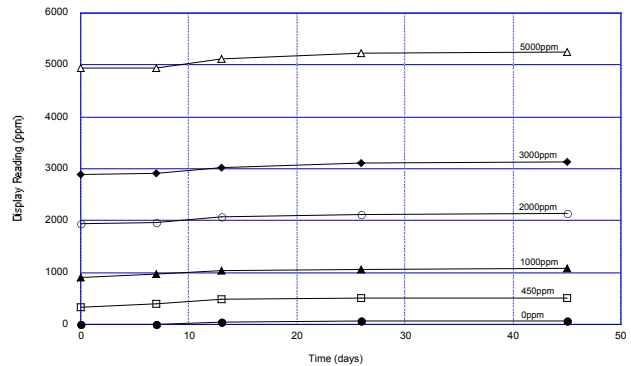
Fig. 9-1 - Durability of FG-010 to high temperature (60°C)
