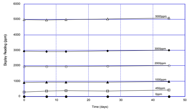
Fig. 9-2 - Durability of FG-010 to low temperature (-10°C)
