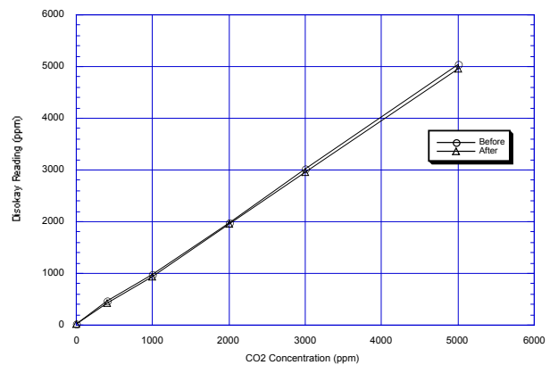
Fig. 8 - Durability of FG-010 to temperature cycling
