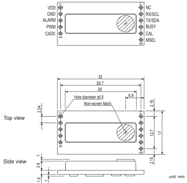
Fig. 3 - Dimensions of FG-010
