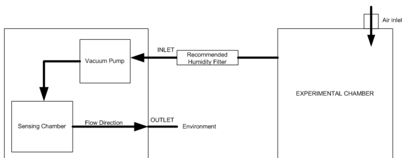
Figure 6: Opened-loop configuration (with environmental exhaust)
