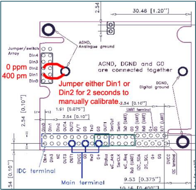
Figure 16: Output and calibration output layout for 1% CO2 K30 sensor
