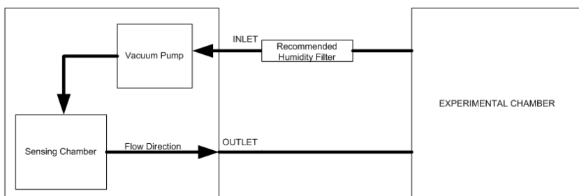
Figure 5: Closed-loop configuration
