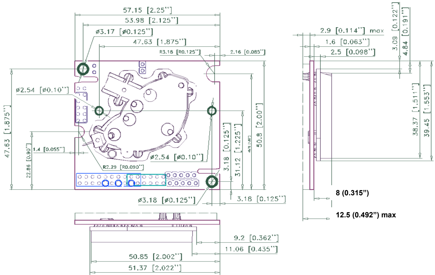
Figure 4. CO 2 Engine® K30 FR mechanical drawing.
