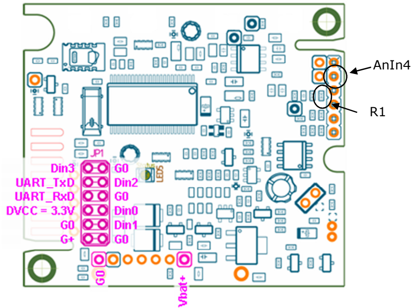
Figure 4, Different connectors
